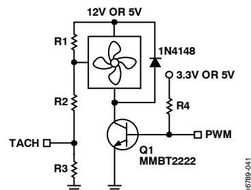
Figure 42. Planning for 3-Wire Fans on a PCB
