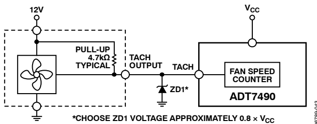
Figure 44. Fan with TACH Pull-Up to Voltage > 3.6 V, for Example, 12 V Clamped with Zener Diode
