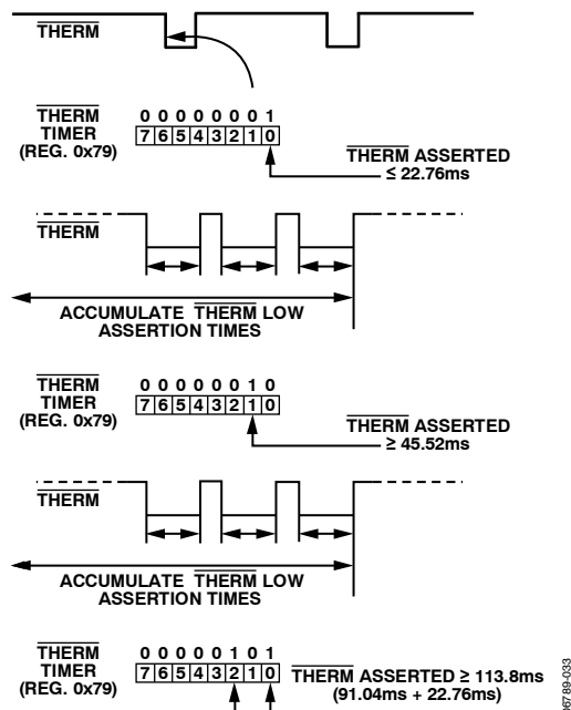
Figure 34. Understanding the THERM Timer
