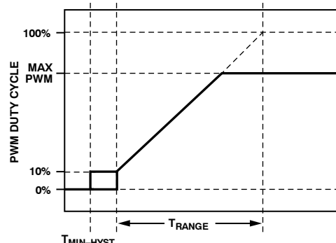
Figure 57. Changing PWM Max Does Not Change the AFC Slope
