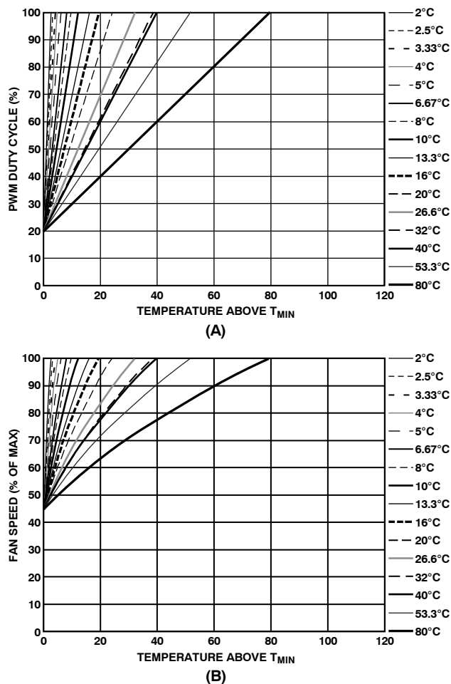
Figure 59. T RANGE and % Fan Speed Slopes with PWM MIN = 20%
