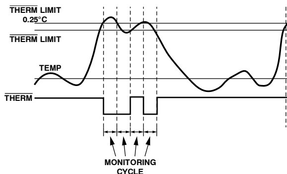
Figure 36. Asserting THERM as an Output, Based on Tripping THERM Limits
