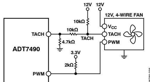
Figure 39. Driving a 4-Wire Fan
