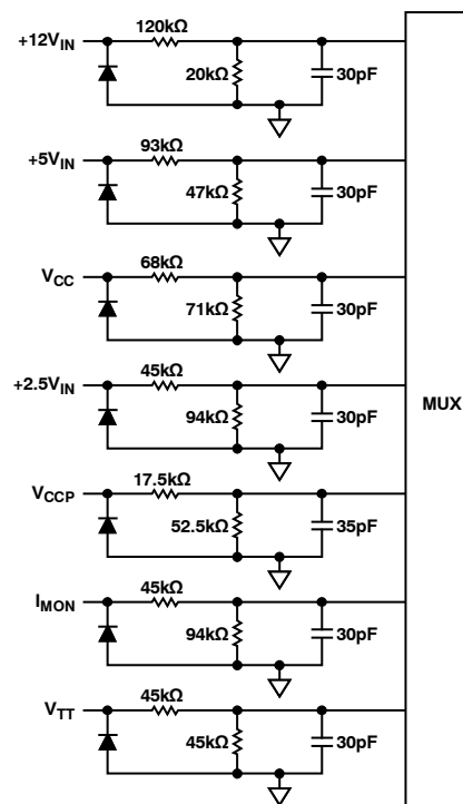
Figure 25. Analog Inputs structure
