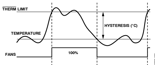
Figure 30. THERM Temperature Limit Operation
