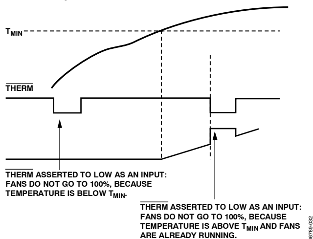
Figure 33. Asserting THERM Low as an Input in Automatic Fan Speed Control Mode
