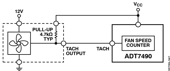
Figure 43. Fan with TACH Pull-Up to V_{CC}
