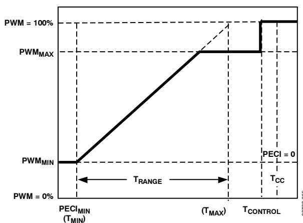
Figure 18. Overview of Automatic Fan Speed Control Using PEGI Thermal Information
