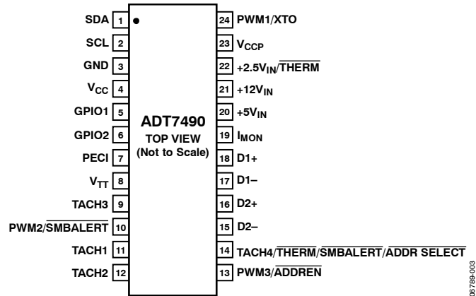
Figure 3. Pin Configuration
