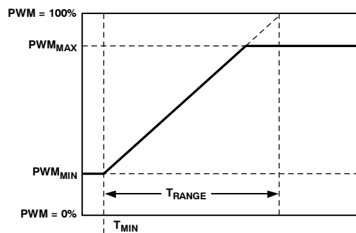
Figure 48. T RANGE
