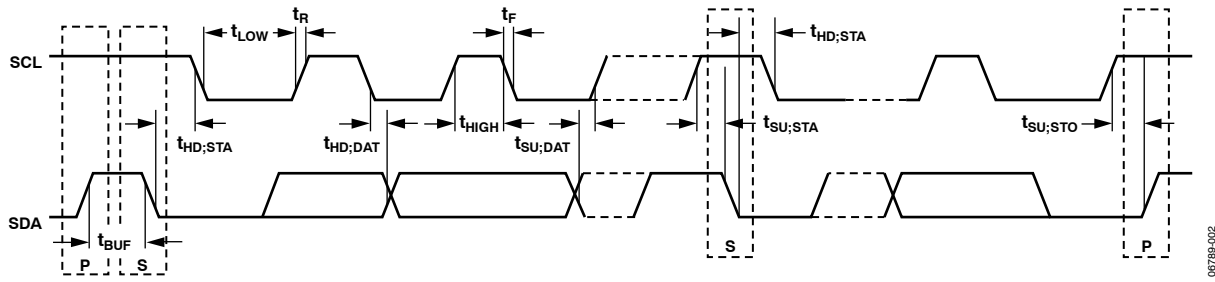
Figure 2. SMBus Timing Diagram
