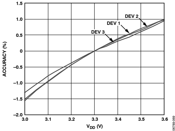
Figure 16. TACH Accuracy vs. Supply Voltage
