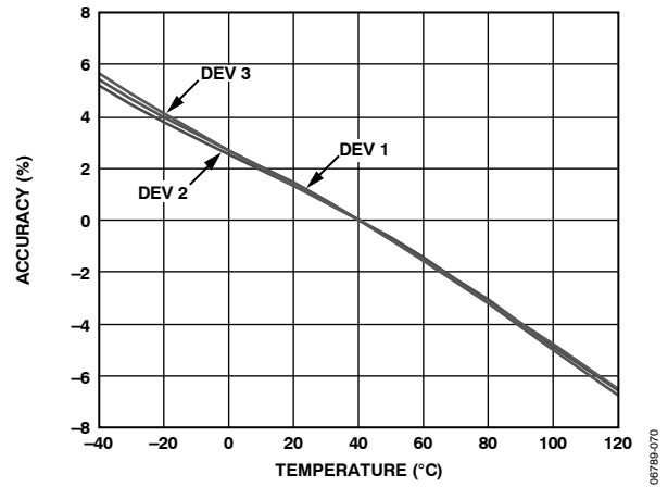
Figure 17. TACH Accuracy vs. Temperature
